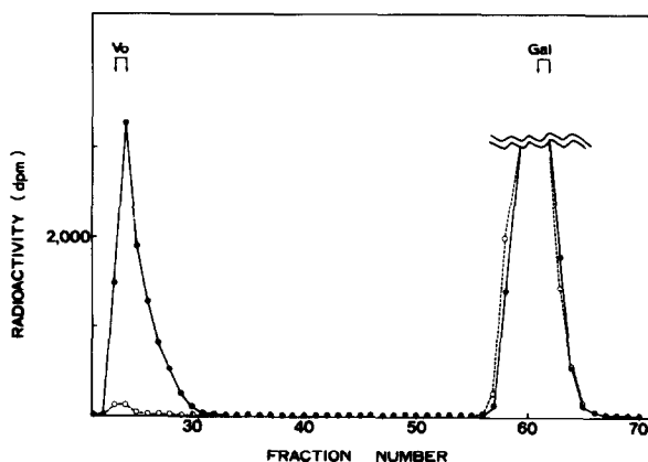
Fig.2. Enzymatic transfer of fucose from GDP-[ ^{14}\text{C} ]fucose to embryoglycan. The reaction was carried out as described in section 2 using 160 \mu g of the enzyme protein and 50 \mu g embryoglycan as the acceptor. The product was analyzed on a column of Sephadex G-50 (1.8 \times 91 cm) equilibrated and eluted with 0.05 M ammonium acetate buffer, pH 6.0. Fractions, 3 ml were collected. Vo and Gal represent the area where blue dextran or galactose was eluted. (●—●) Experimental run; (○---○) control run in which embryoglycan was not added to the reaction mixture.
